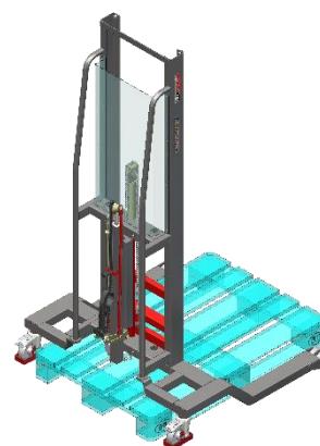
Pallet hanger
